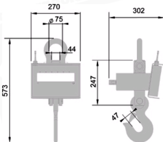
MCWK: Dimensions in mm.
