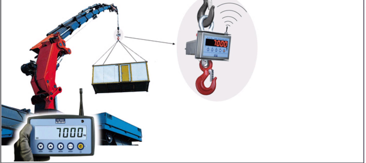
DFWPM: Single scale weight repeater application.
