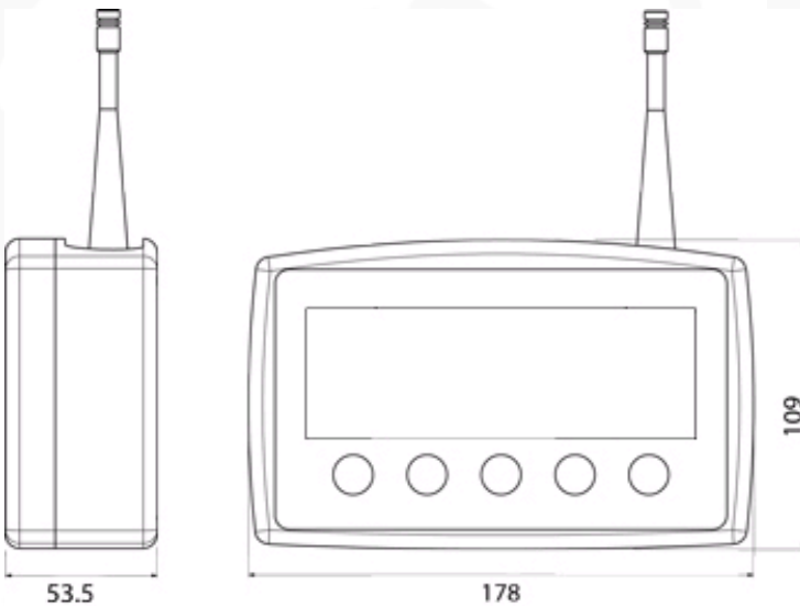
DFWPM: dimensions in mm.
